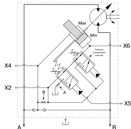
HPC control, type M, negative control (begins at max. displacement)
