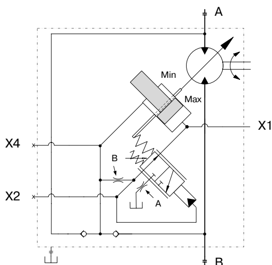
ACI control, type T, positive control (begin in min. displacement)
