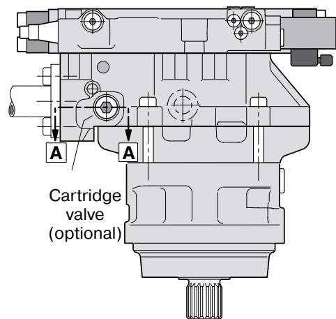
V14- 110 (EP control) with relief valve cartridges.
