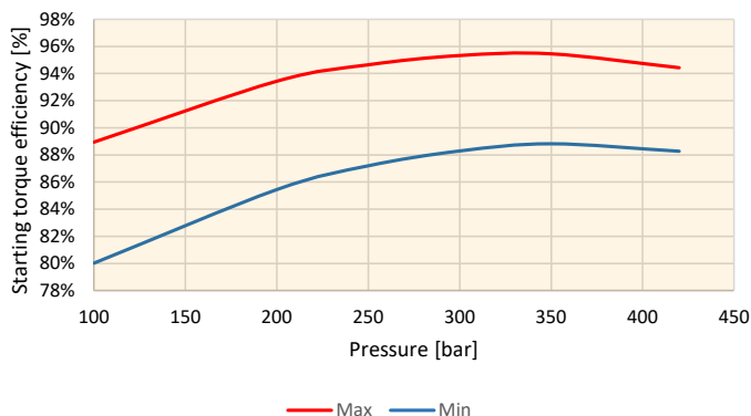
V16-220 limited displacement = 180 cc/rev
