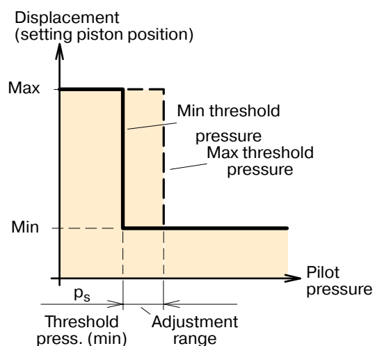
HO diagram (displacement vs. pilot pressure).
