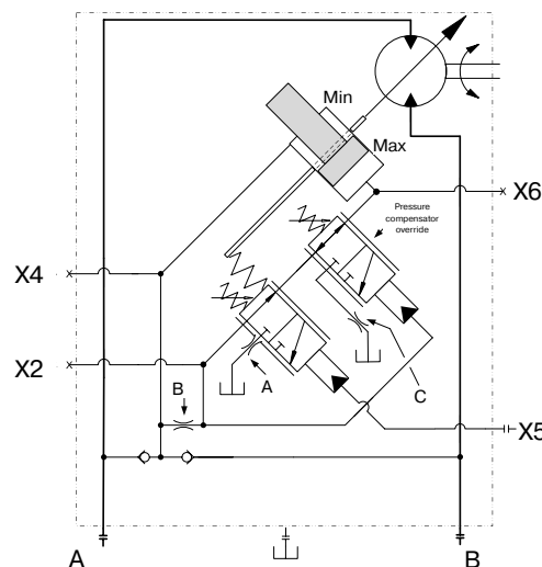
HPC control, type T, positive control (begins at min. displacement)
