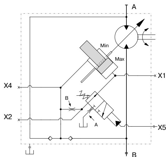
HO control, type T, positive control (begins at min. displacement)
