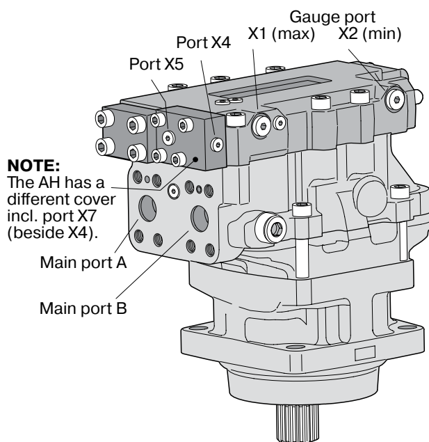
Port locations – V14- with AC or AH compensator.
