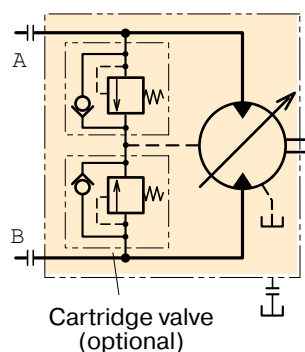
Hydraulic schematic
