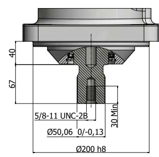
Shaft code U, -270
