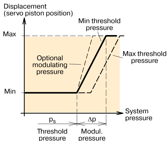
AC diagram (displacement vs. system pressure).
