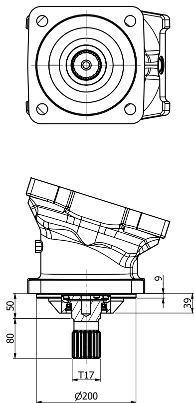
270, T17 ISO Bearing housing
