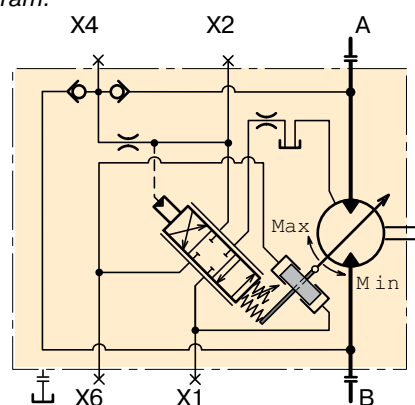
ACI 01 I schematic (spool in a balanced, mid-pos.).
