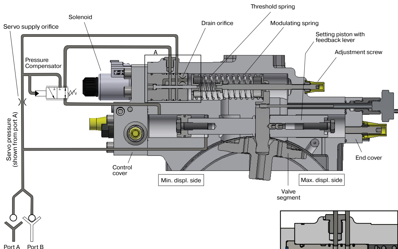
EPA/EPB control function (displ. increases at decreasing solenoid current), negative control (M* code).
