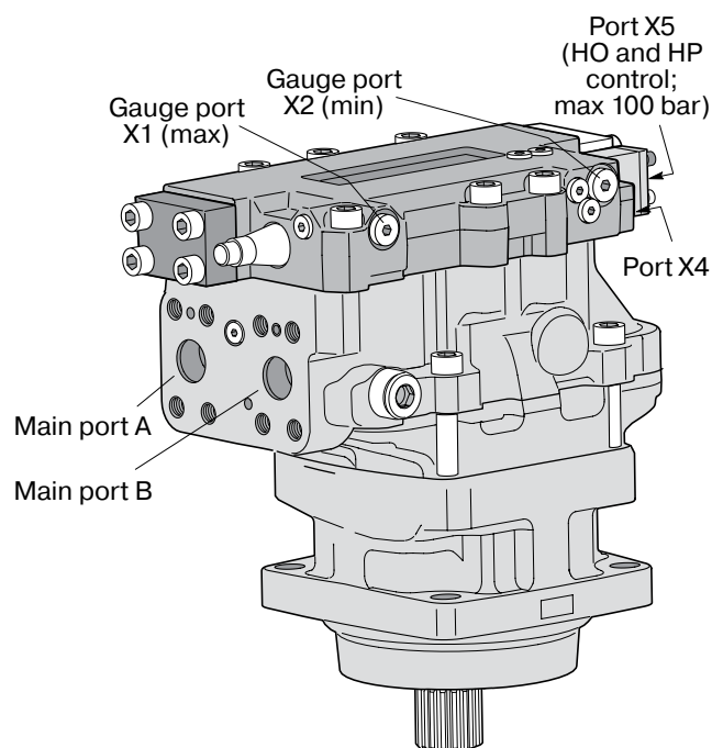
Port locations – V14- 110 with HO or HP control.
