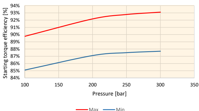
V16-270 limited displacement = 220 cc/rev
