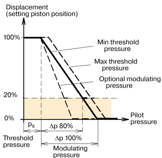
HP diagram (displacement vs. pilot pressure). (type M, negative control)
