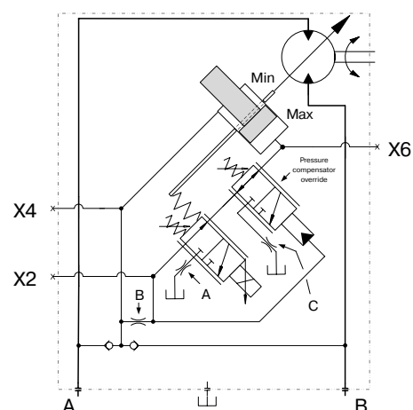
EPA/B control, type T, positive control (begins at min. displacement)
